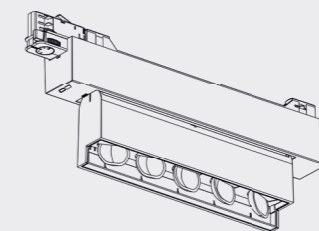
TRACK 395 x 50 mm | H: 130 mm
